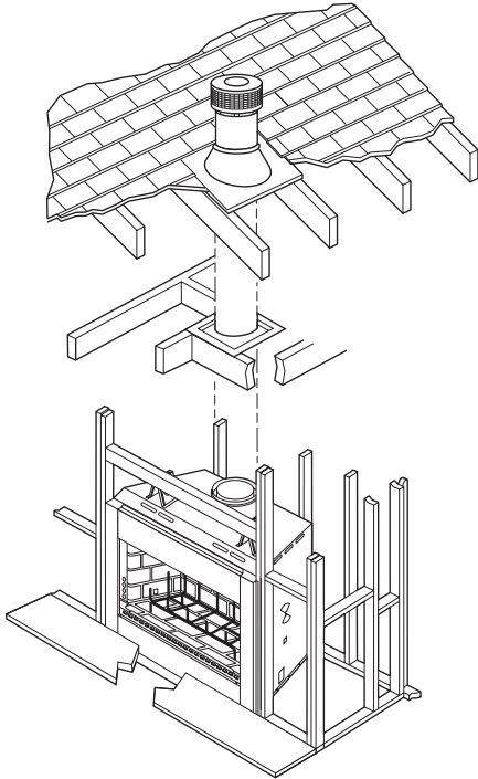
Typical Installation
