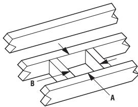
Ceiling Framing
